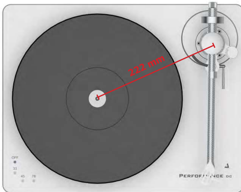
Pic. 10: Distance from pivot to spindle
