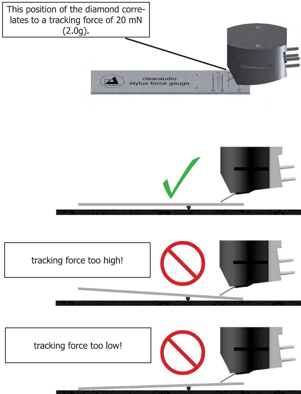
Pic. 12: Use of Smart Stylus Gauge
