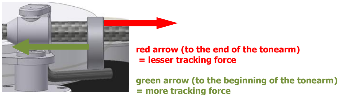
Pic. 12: Adjustment of the Tracking force
